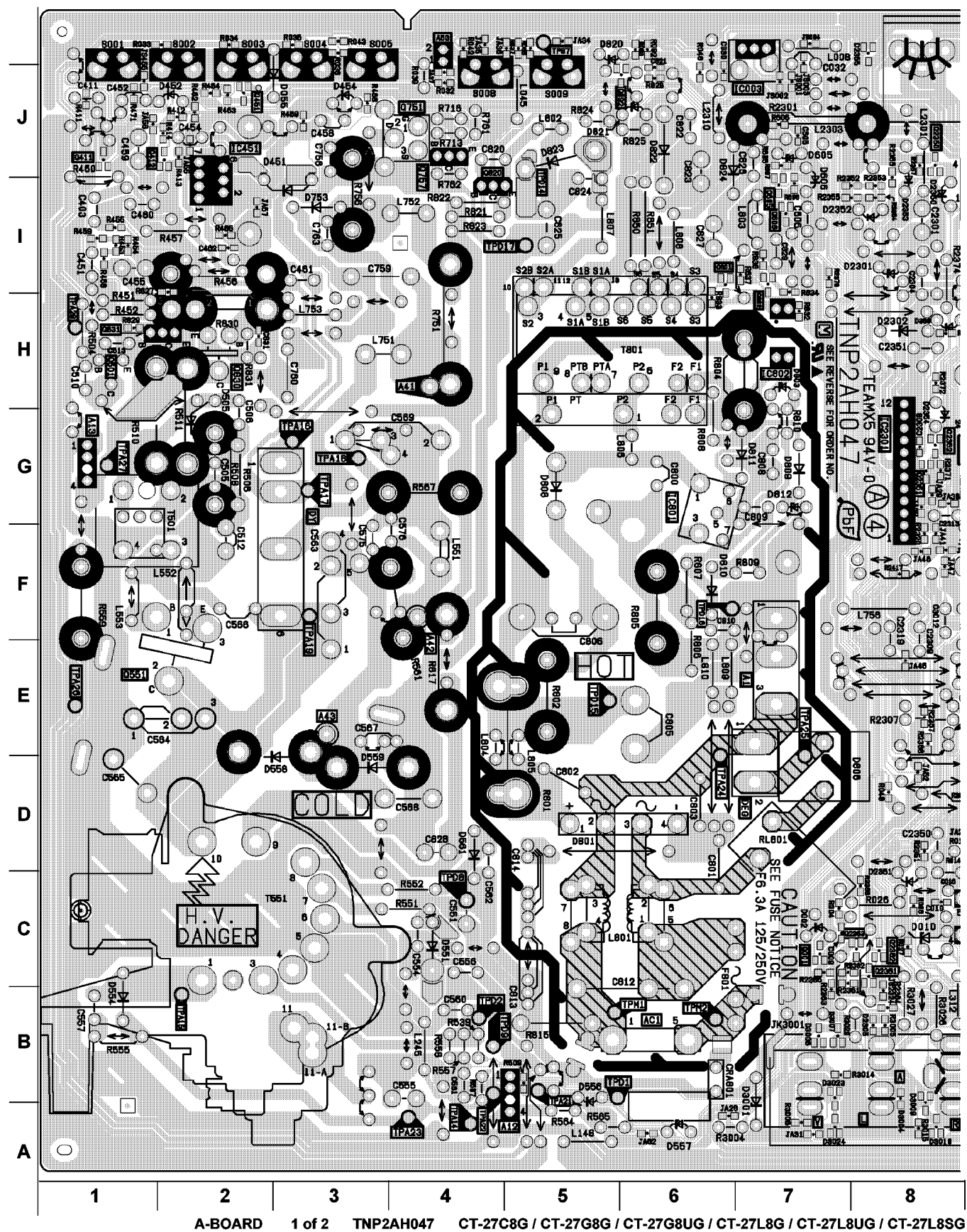
A-BOARD 1 of 2 TNP2AH047 CT-27C8G / CT-27G8G / CT-27G8UG / CT-27L8G / CT-27L8UG / CT-27L8SG
