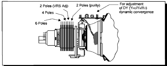
Convergence Magnets and Wedges Location
