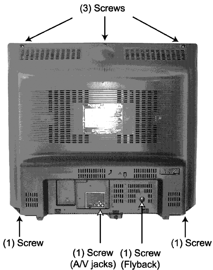
Back Cover (CT-27L8G/UG/SG, CT-27G8G/UG)
