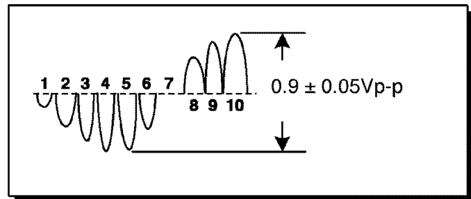
TP35 Waveform.
