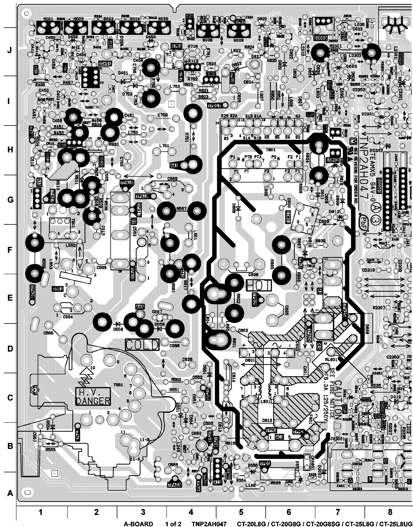
A-BOARD 1 of 2 TNP2AH047 CT-20L8G / CT-20G8G / CT-20G8SG / CT-25L8G / CT-25L8UG
