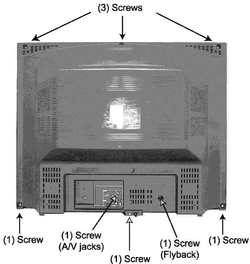
Back Cover (CT-27C8G).
