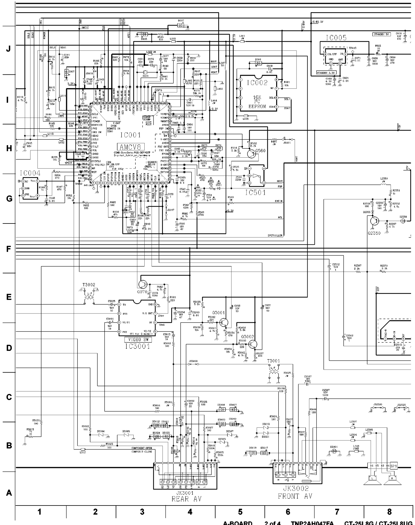
A-BOARD 2 of 4 TNP2AH047FA CT-25L8G / CT-25L8UG
