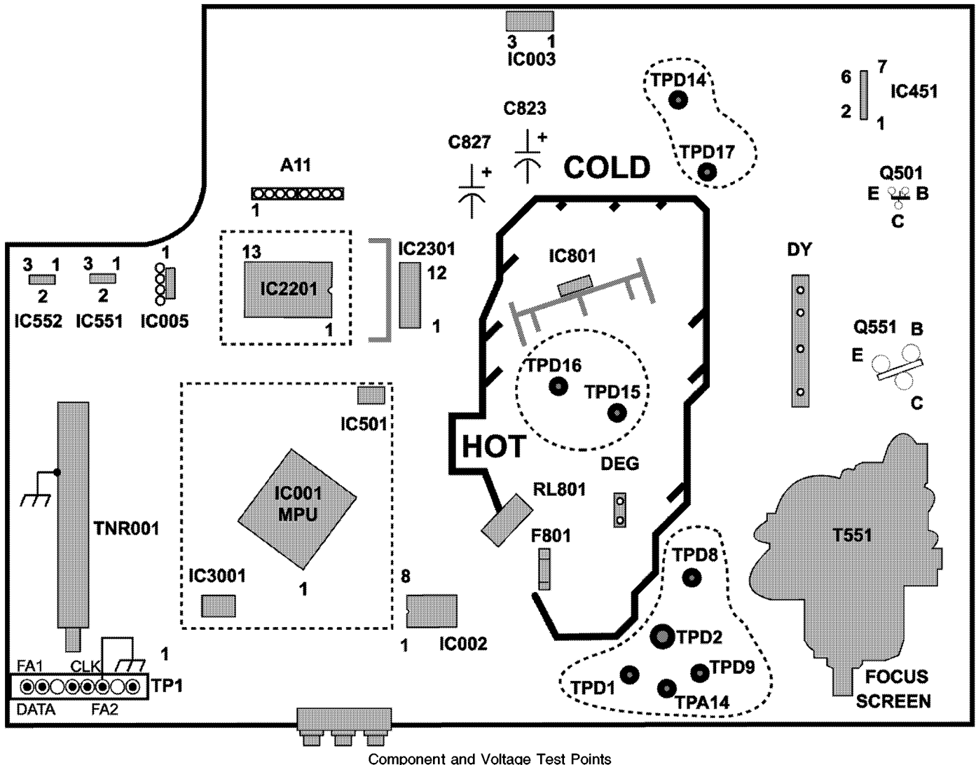
Component and Voltage Test Points
