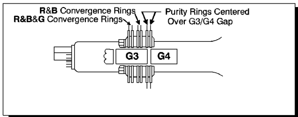
2 piece assembly
