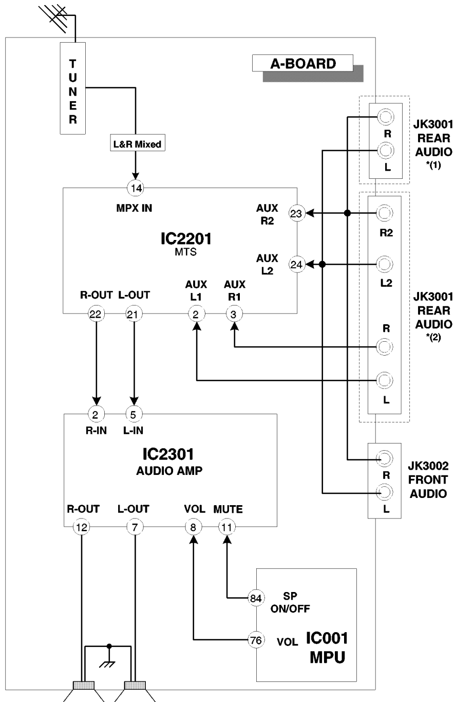
Audio signal path block diagram
