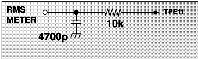
Filter Jig
