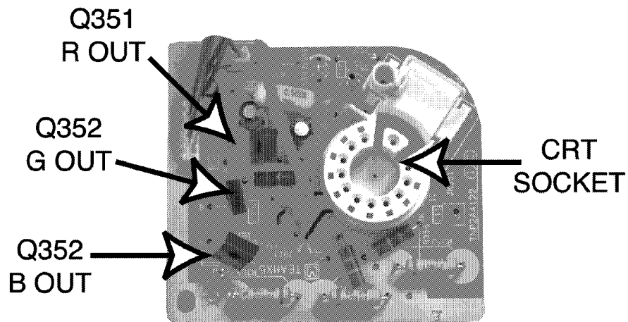
C-Board component locations
