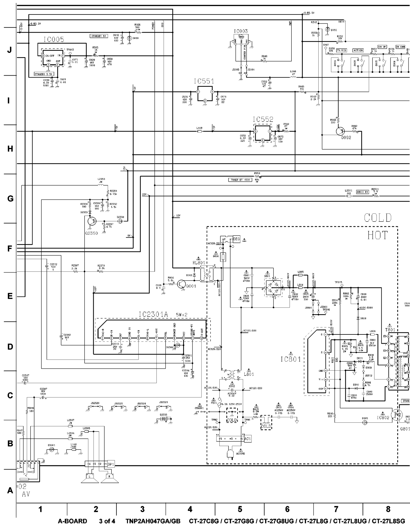
A-BOARD 3 of 4 TNP2AH047GA/GB CT-27C8G / CT-27G8G / CT-27G8UG / CT-27L8G / CT-27L8UG / CT-27L8SG
