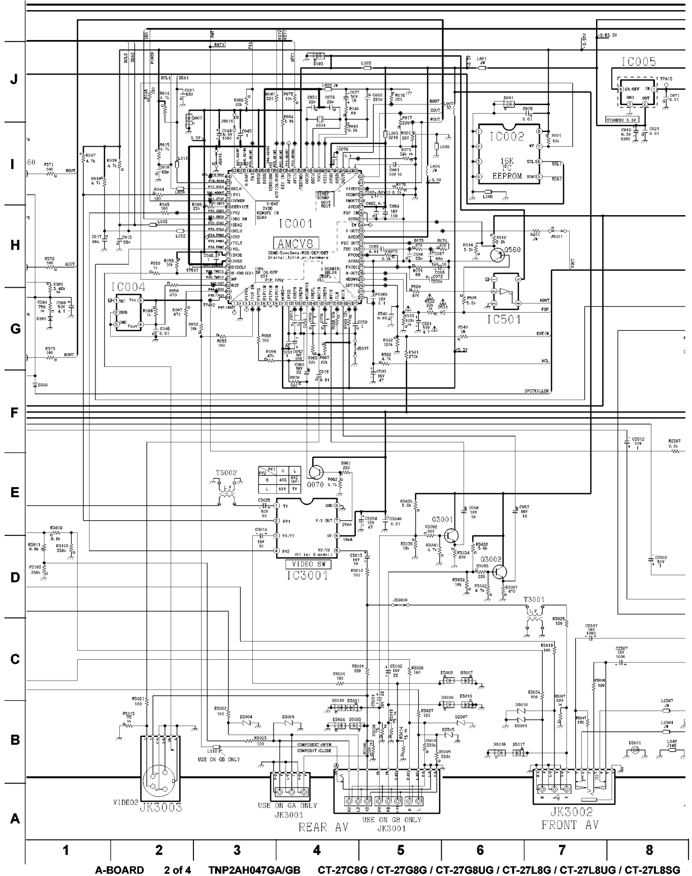
A-BOARD 2 of 4 TNP2AH047GA/GB CT-27C8G / CT-27G8G / CT-27G8UG / CT-27L8G / CT-27L8UG / CT-27L8SG
