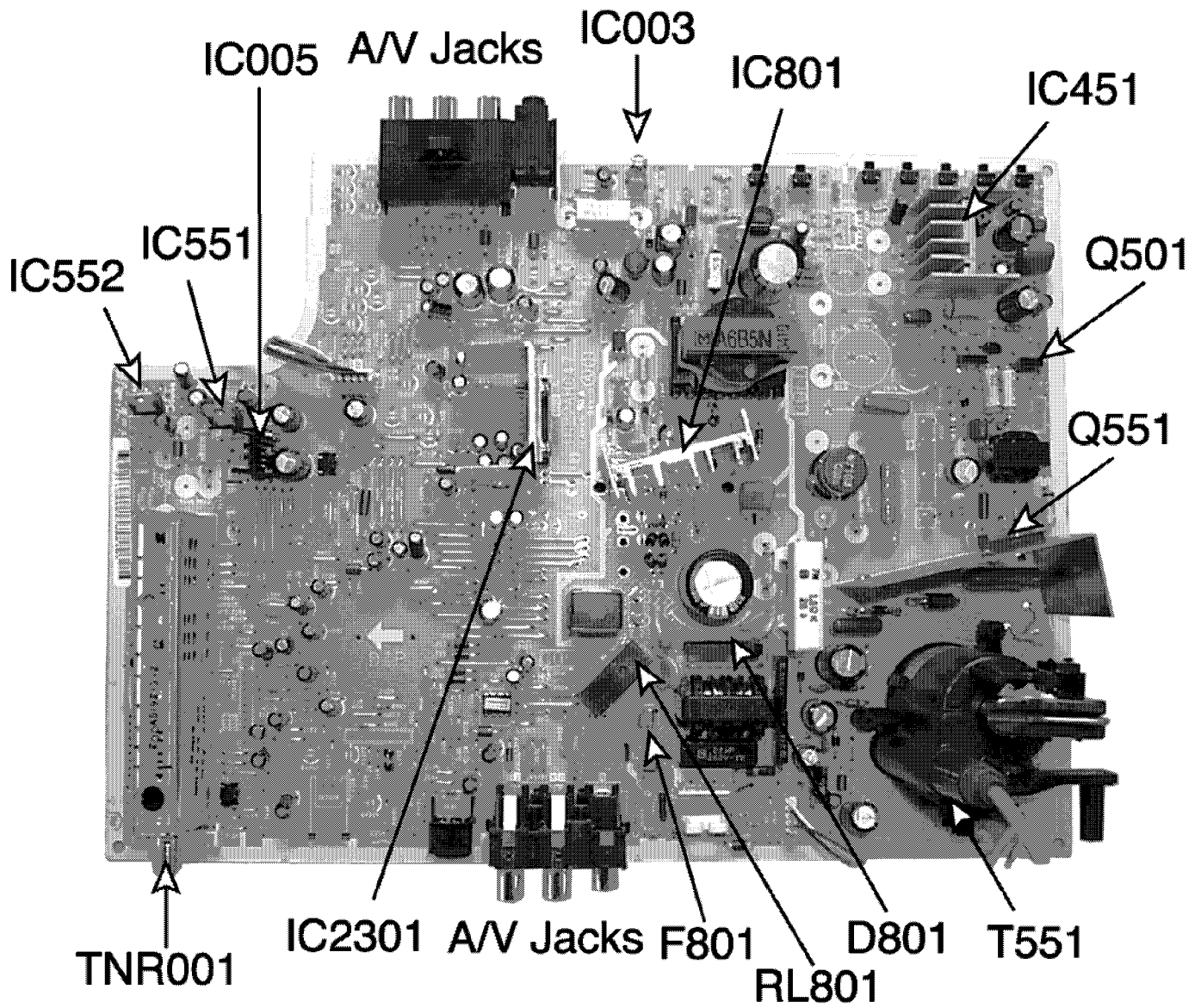
A-Board chassis (Top view)
