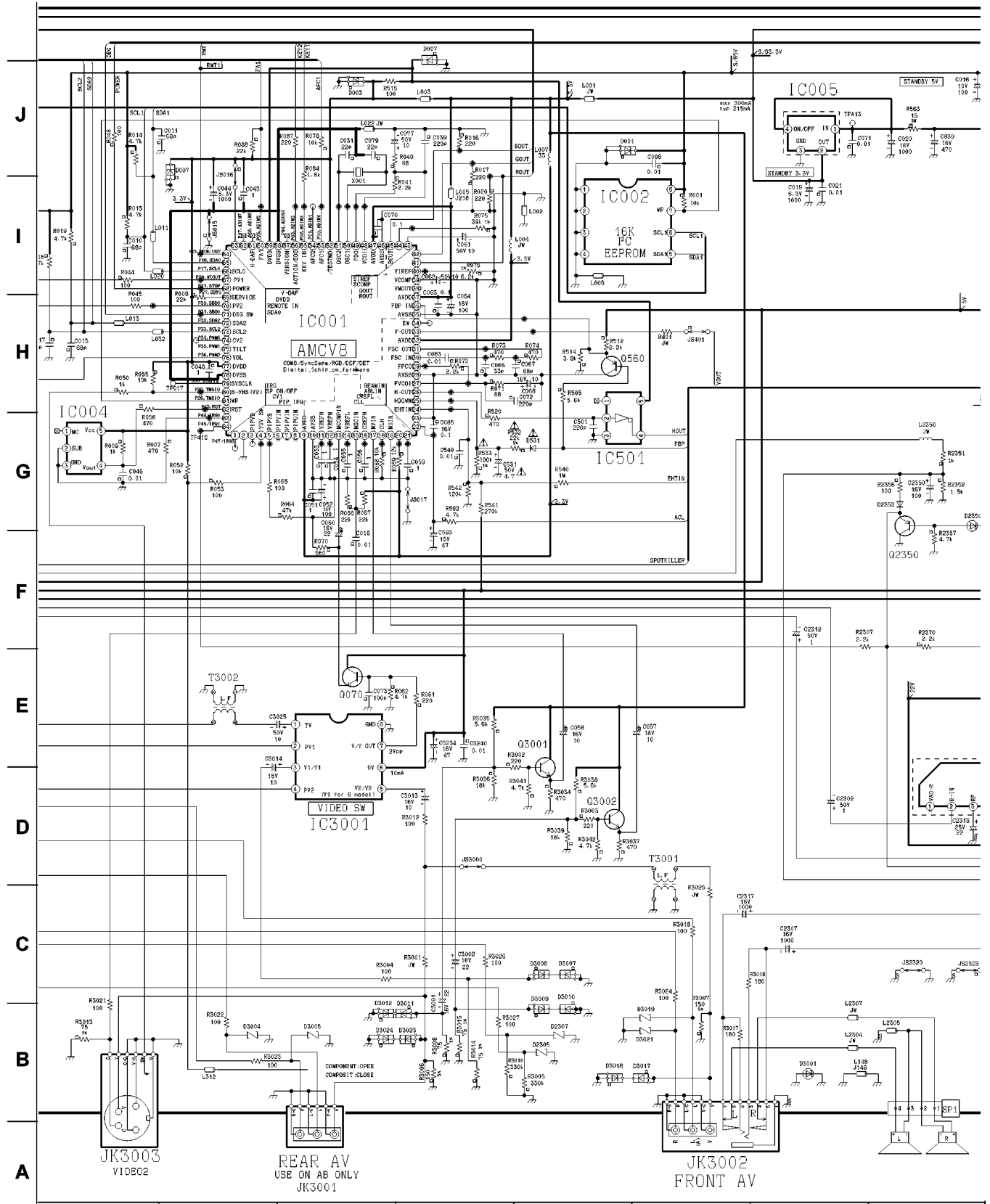
1 2 3 4 5 6 7 8 A-BOARD 2 of 4 TNP2AH047AA/AB CT-20L8 / CT-20G8 / CT-20G8S
